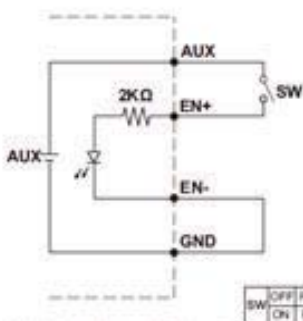
(A) Using internal 5V auxiliary source
