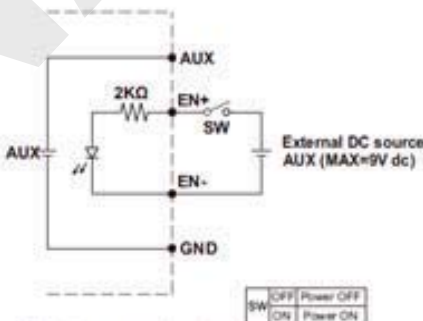
(C) Using external voltage source
