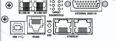
Rear communication interfaces with EtherCAT (+ECAT) option.
